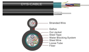
GYTC8S Outdoor Cable
