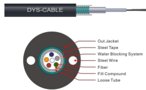
GYXTW Outdoor Cable
