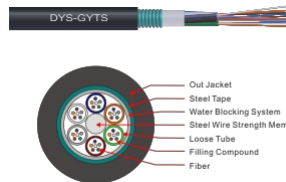
GYTS Outdoor Cable
