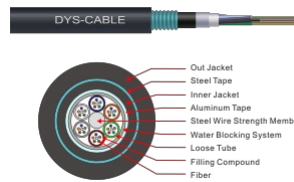
GYTA53 Outdoor Cable
