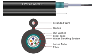
GYXTC8S Outdoor Cable
