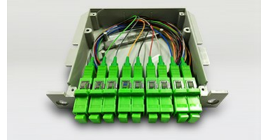
1X8 LGX PLC splitter with SC APC connector
